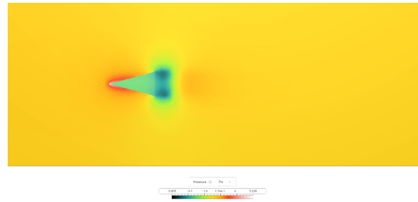
Figure B.6: Pressure distribution for the 30° cone ( k - \epsilon model).
