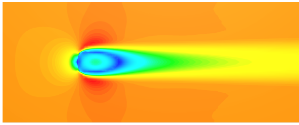
Figure B.20: Velocity magnitude contour for the 150° cone, exhibiting the largest wake deficit.
